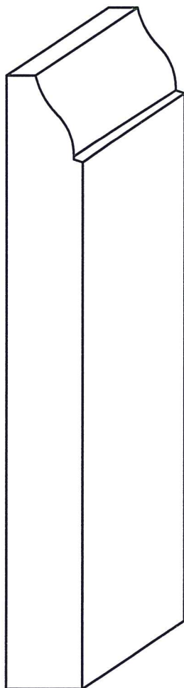
314MUL-4 9/16 X 4 1/2
