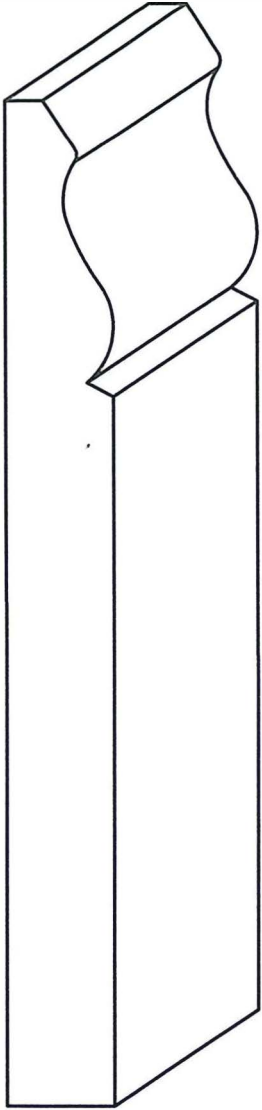
328MUL-5 9/16 X 5 1/4
